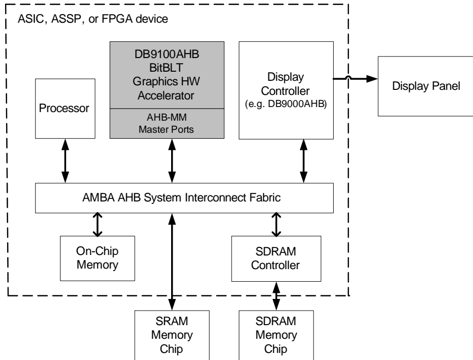
Figure 1: DB9100AHB BitBLT Graphics HW Accelerator – System Diagram
